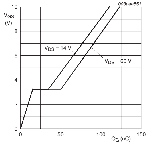
T_j = 25^\circ\text{C}; I_D = 25 A Fig 14. Gate-source voltage as a function of gate charge; typical values
