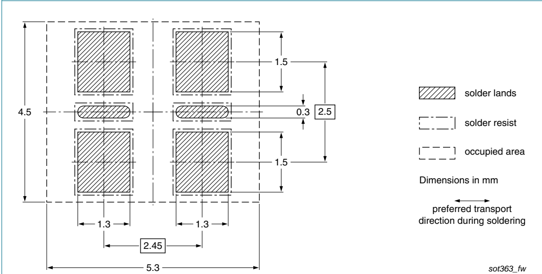
Fig 20. Wave soldering footprint SOT363 (SC-88)
